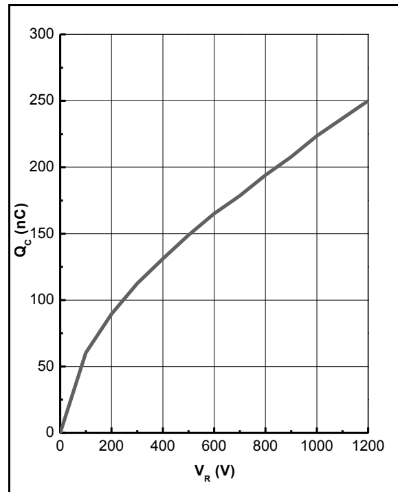
Figure 4. Total Capacitance Charge vs. Reverse Voltage
