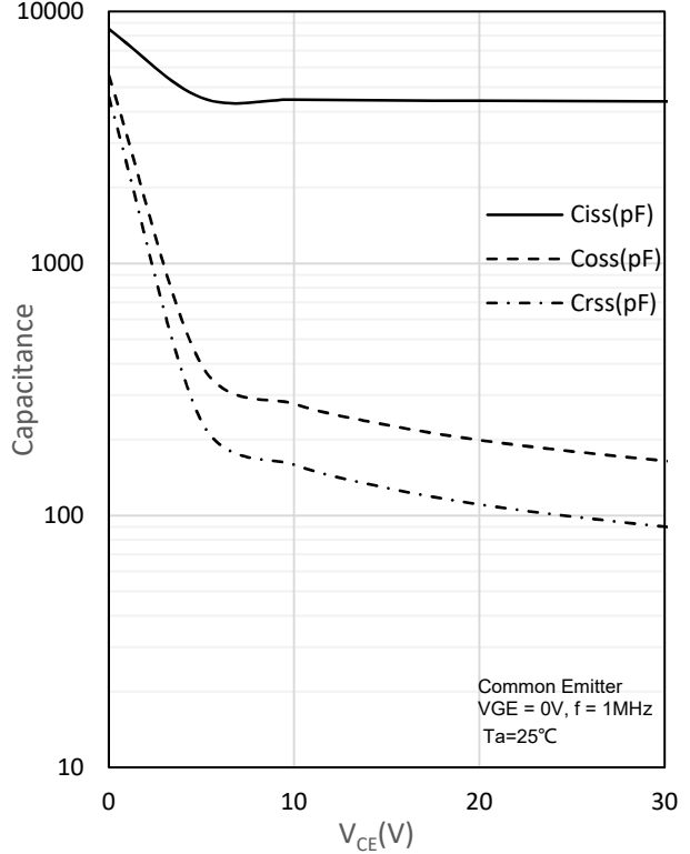
Fig. 12 Capacitance characteristics
